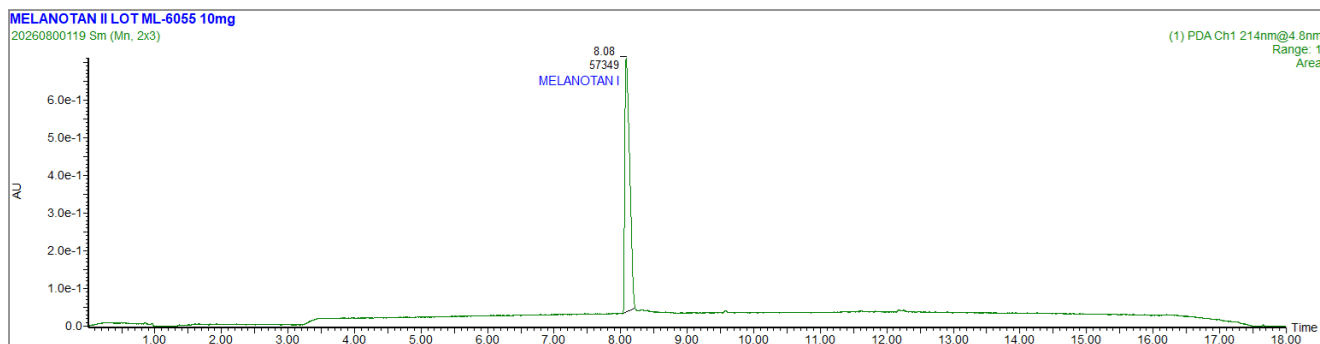
UV CHROMATOGRAM
