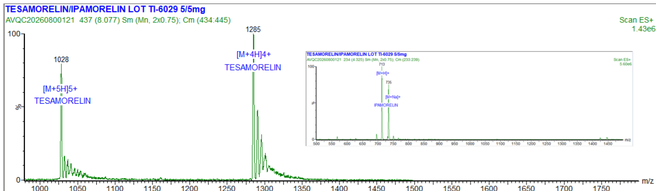
MASS SPECTRUM / SPECTRA
