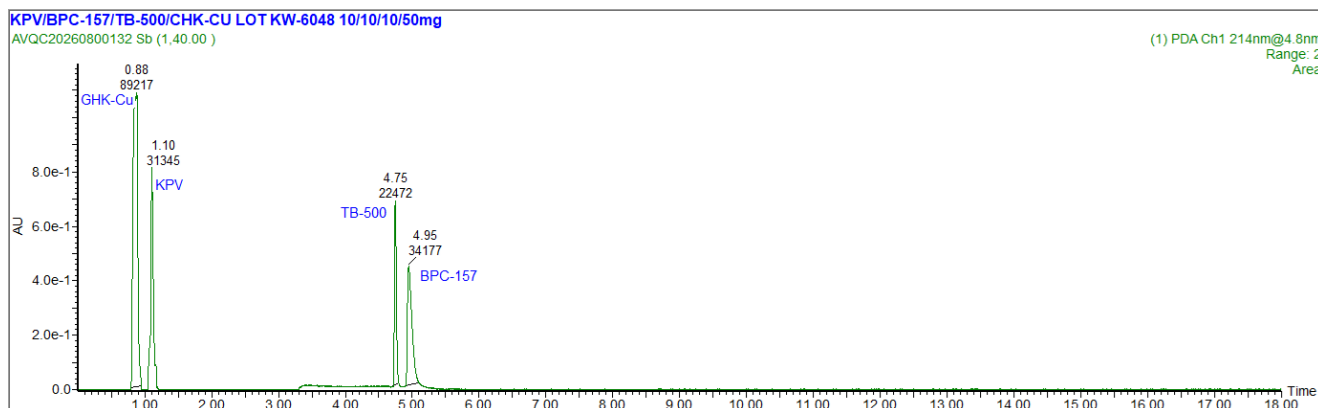
UV CHROMATOGRAM
