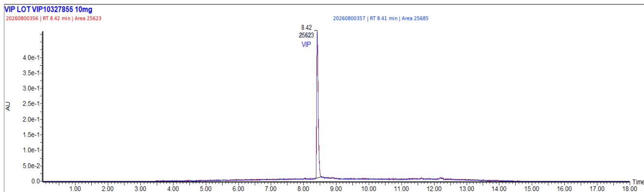
UV CHROMATOGRAM
