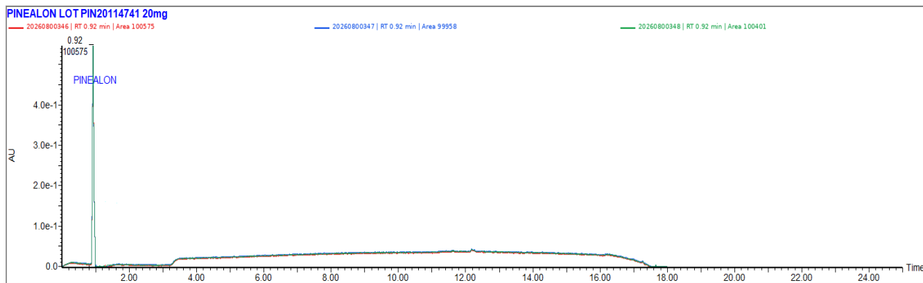
UV CHROMATOGRAM
