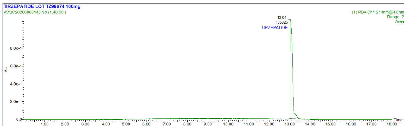
UV CHROMATOGRAM
